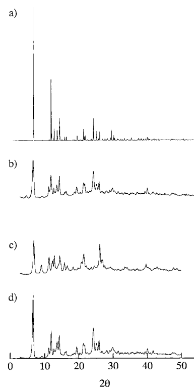
Figure 3. a) Simulated XRPD pattern upon removal of the water molecules from the single crystal. Observed XRPD patterns of as-synthesized sample 1 (b), anhydrous sample 2 (dried at 110 °C under reduced pressure for 5 h) (c), and MeOH immersed sample after drying (d)
